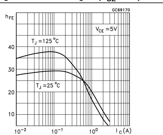
Figure 7. DC current gain ( V_{CE} = 5 V)
