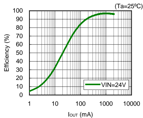
R1243x001C/R1243x001D
