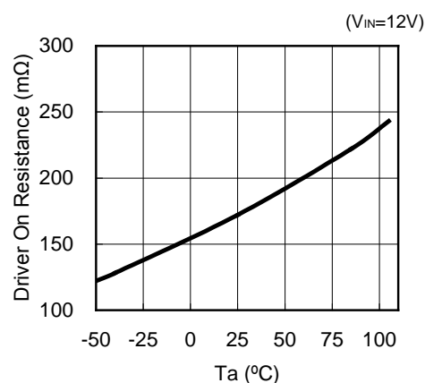
R1243x001x
