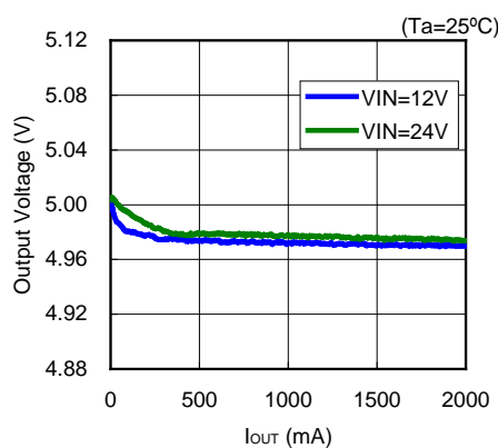
R1243x001A/R1243x001B, R1243S001E
