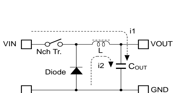
Basic Circuit
