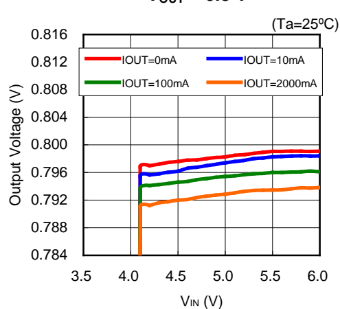
R1243x001C/R1243x001D
