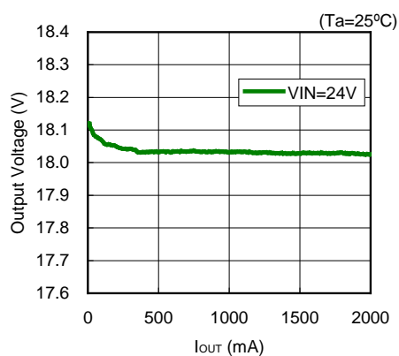
R1243x001A/R1243x001B, R1243S001E
