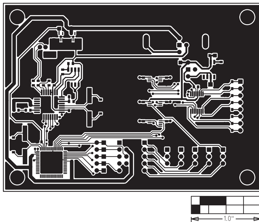
Figure 6. MAX5258 EV Kit PCB Layout—Component Side
