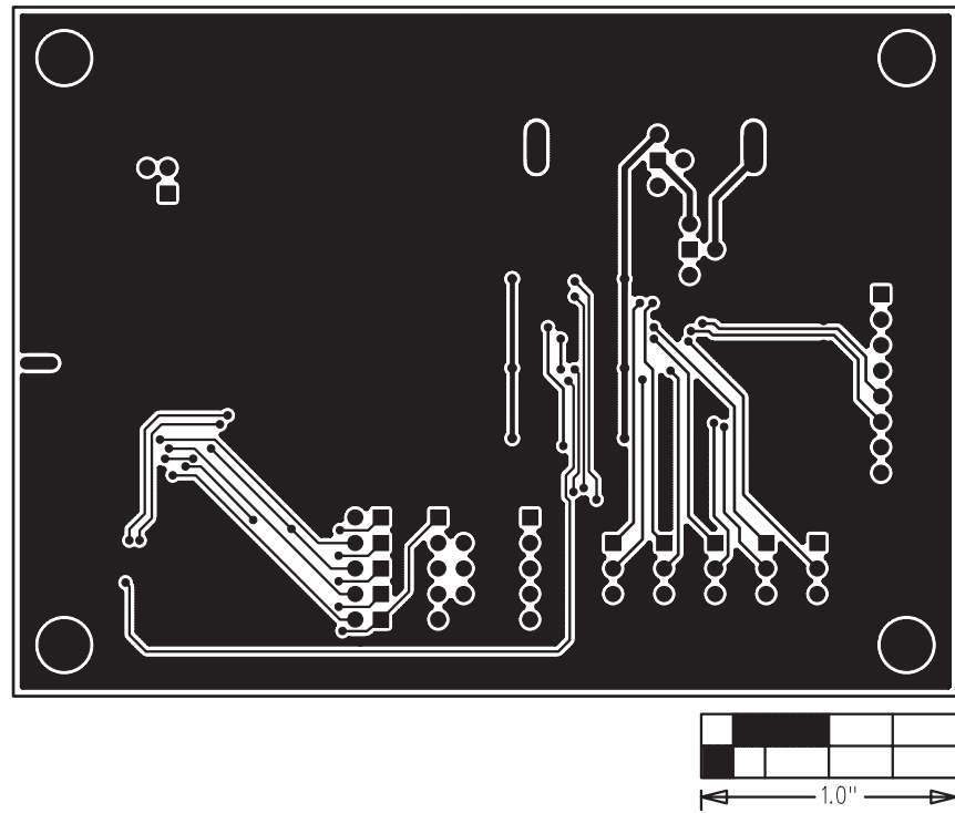
Figure 7. MAX5258 EV Kit PCB Layout—Solder Side
