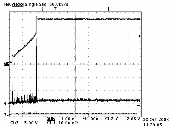
Figure 11. DC481 Soft Startup ( R_{LOAD} = 3.3\Omega , V_{IN} = 12\text{V} , V_{OUT} = 3.3\text{V} , T_A = 25^\circ\text{C} ) CH2 is V_{OUT} , CH3 is Power Good, CH4 is I_{IN} (200mA/10.0mVΩ)
