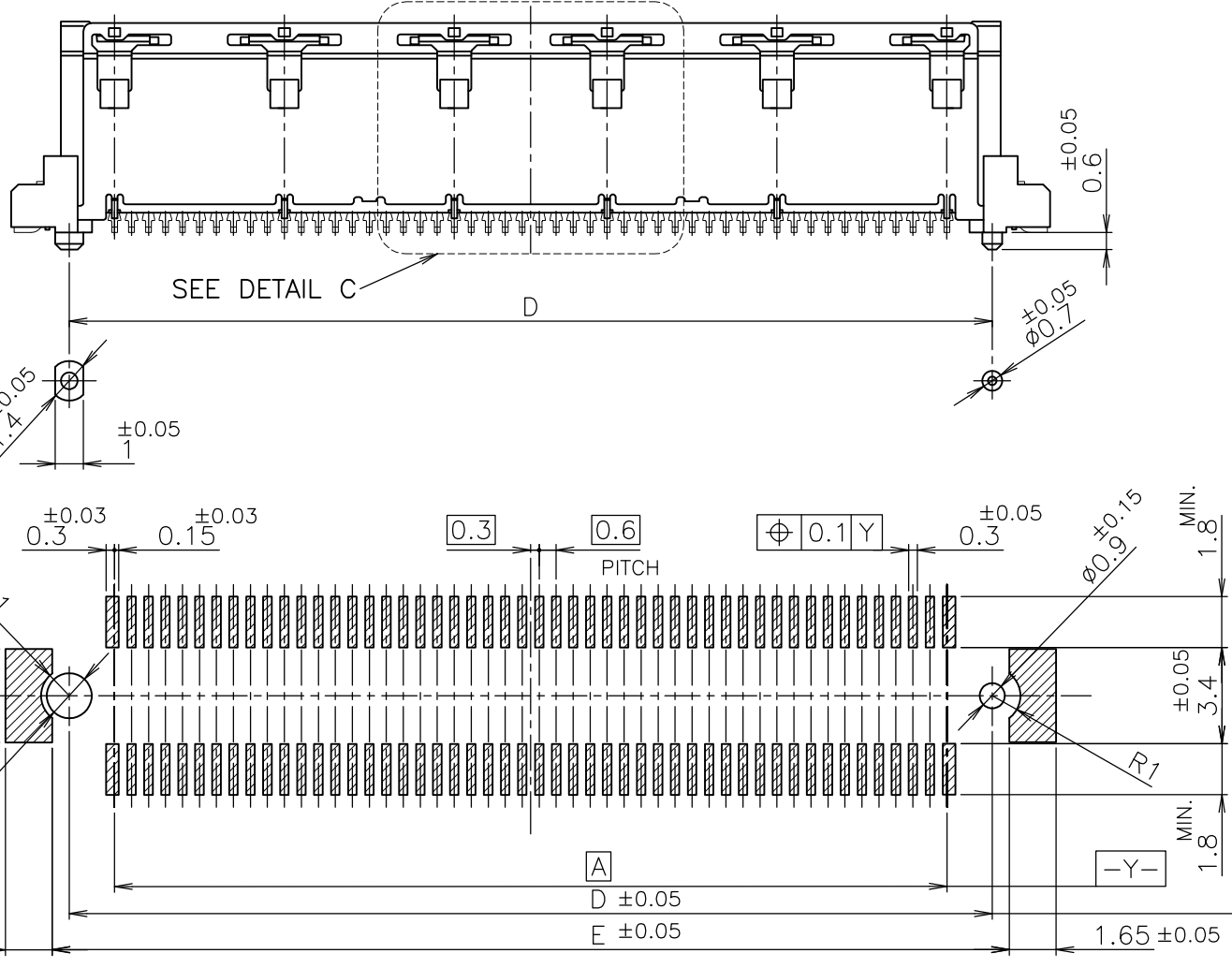
REFERENCE P.C.BOARD LAYOUT
