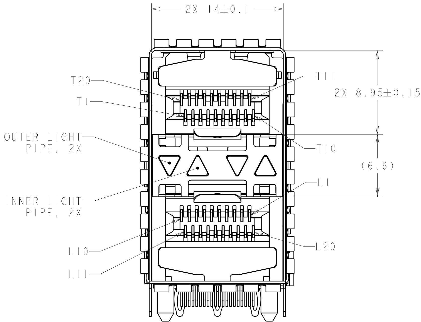
2007492-5 AS SHOWN
