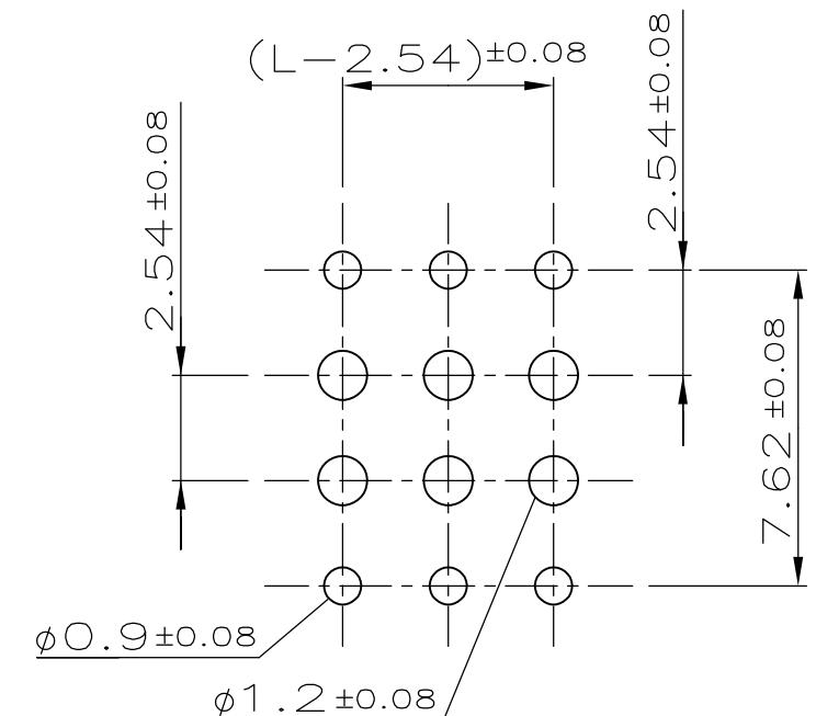
P.C.-BOARD HOLE-PATTERN
