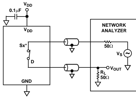
Figure 25. Off Isolation
