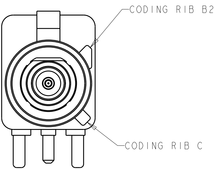
DETAIL H
