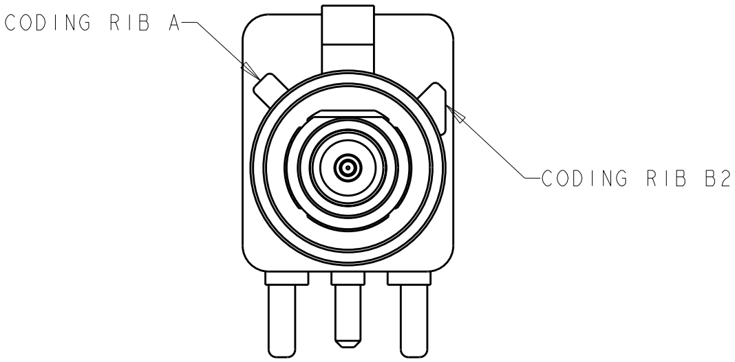
DETAIL B
