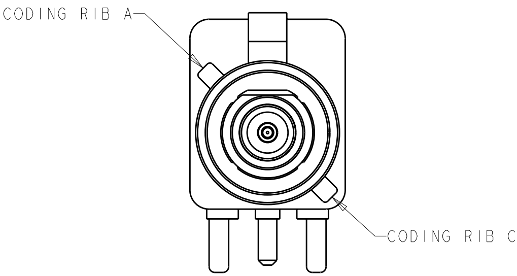
DETAIL C
