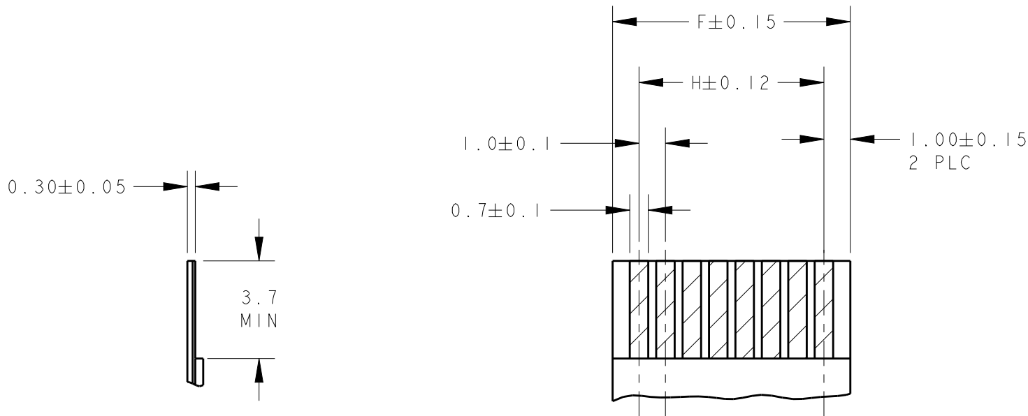
RECOMMENDED FFC/FPC
