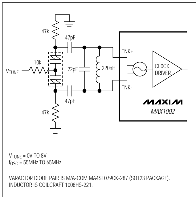
Figure 6. Tank-Resonator Oscillator
