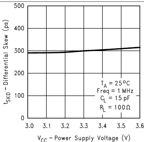
Figure 11. Differential Skew vs Power Supply Voltage
