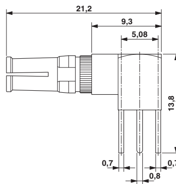
Dimensional drawing
