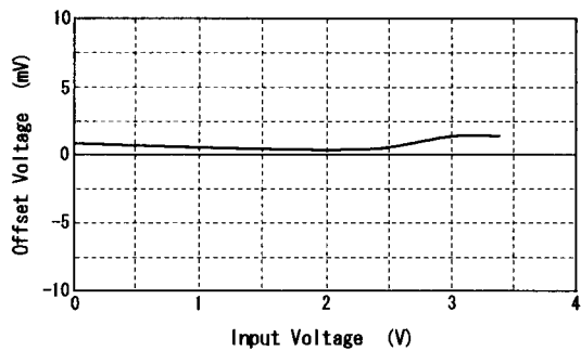
Offset Voltage vs. Input Voltage V_{DD}=3.0V
