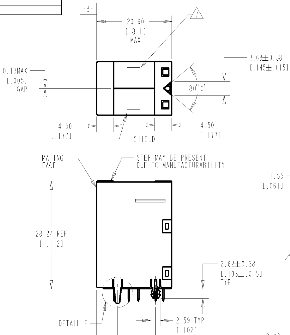
DETAIL F SCALE 8:1
