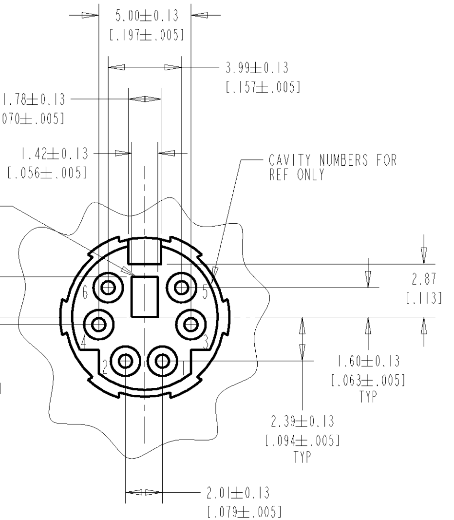
DETAIL D SCALE 5:1
