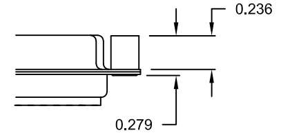
03X..... 0.236" (MATING SIDE) - CN8
