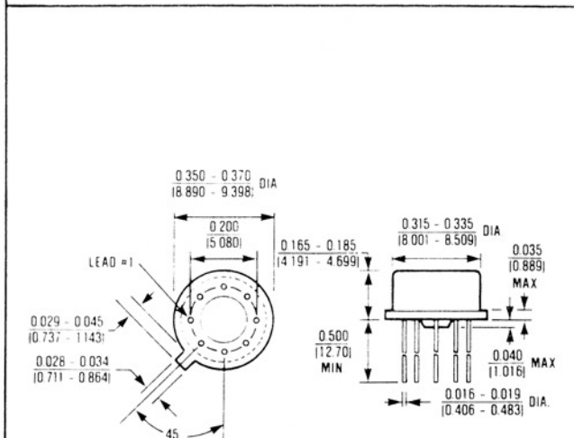
8 Lead TO-99 (TV) \theta_{JA} = 25^{\circ}\text{C/W} \theta_{JC} = 2^{\circ}\text{C/W}
