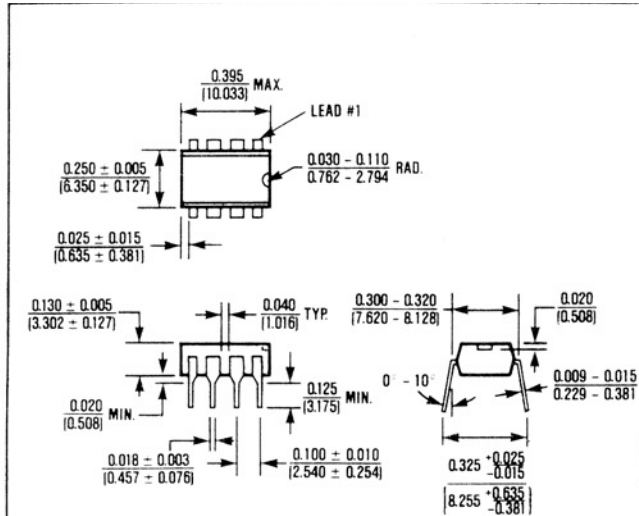
8 Lead Plastic DIP (PA) \theta_{JA} = 160^{\circ}\text{C/W} \theta_{JC} = 75^{\circ}\text{C/W}
