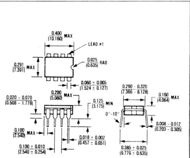
8 Lead Cerdip (JA) \theta_{JA} = 125^{\circ}\text{C/W} \theta_{JC} = 55^{\circ}\text{C/W}
