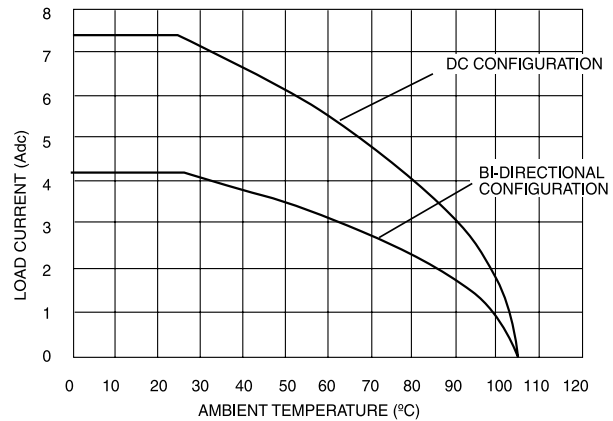
LOAD CURRENT DERATING CURVE (NO HEAT SINK) FIGURE 3
