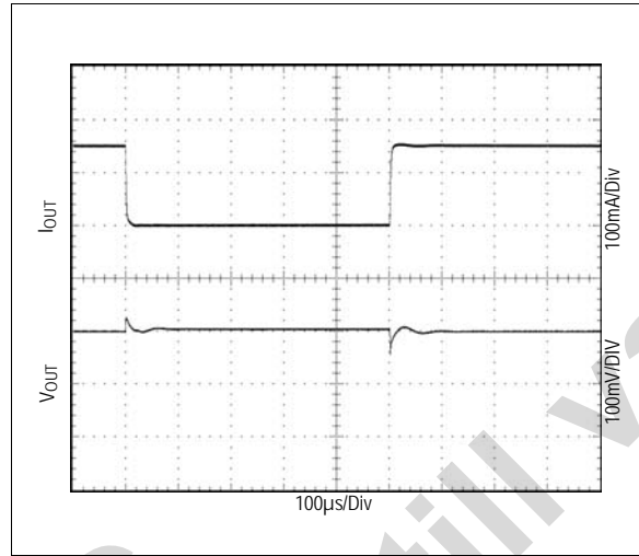
Figure 41. Load Transient; I_{OUT}=0mA to 150mA V_{IN}=3.3V , V_{OUT}=2.8V
