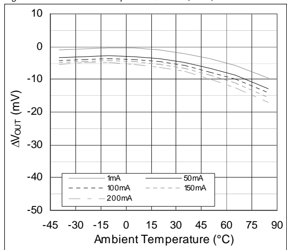
Figure 16. \Delta V_{OUT} vs. Temperature; V_{OUT(NOM)}=2.8V
