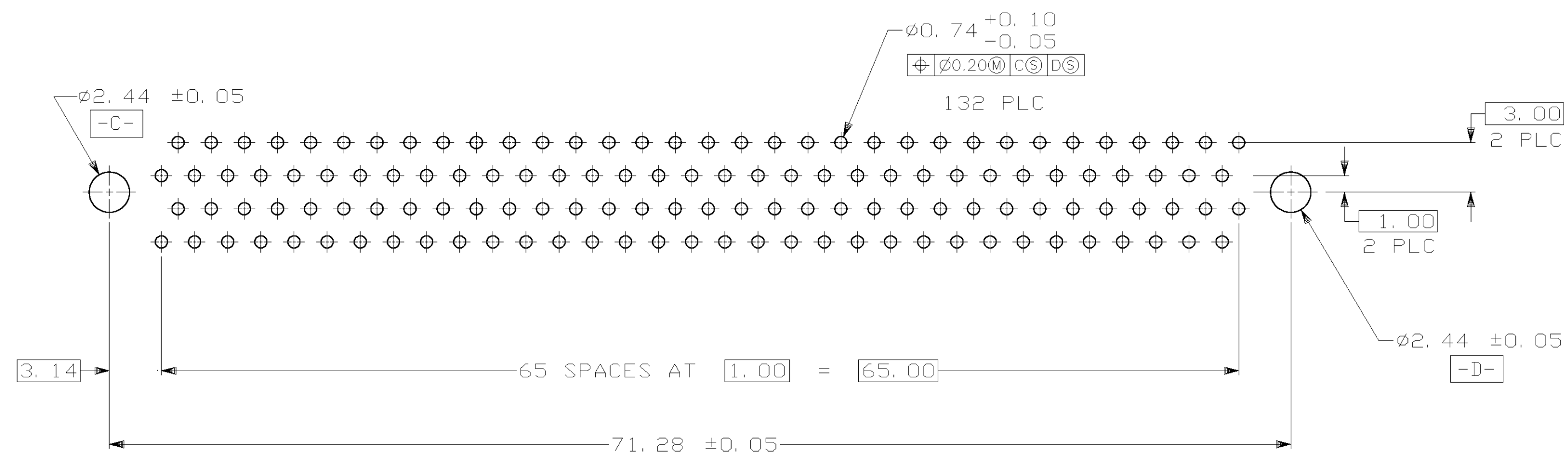
RECOMMENED CONNECTOR MOUNTING HOLE PATTERN (CONNECTOR SIDE SHOWN)
