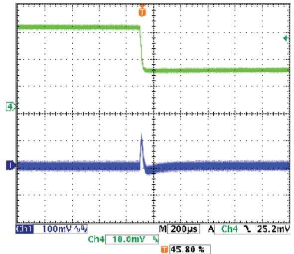
Step Load Transient Response (Vin=5V, Vout=2.5V, Load=0, Iout=16A to 8A) Trace 1=Vout, 100 mV/div. Trace 4=Iout, 5A/div.
