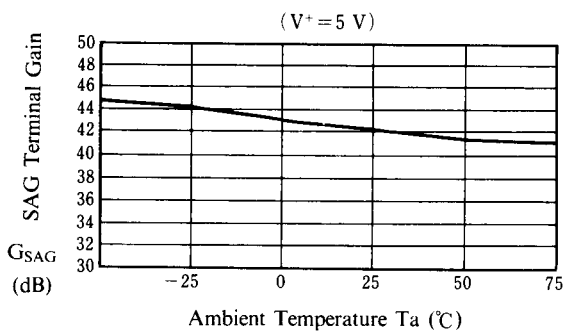
SAG Terminal Gain vs. Ta
