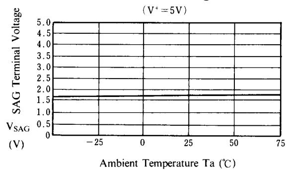
SAG Terminal Voltage vs. Ta
