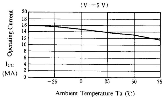
Operating Current vs. Ta
