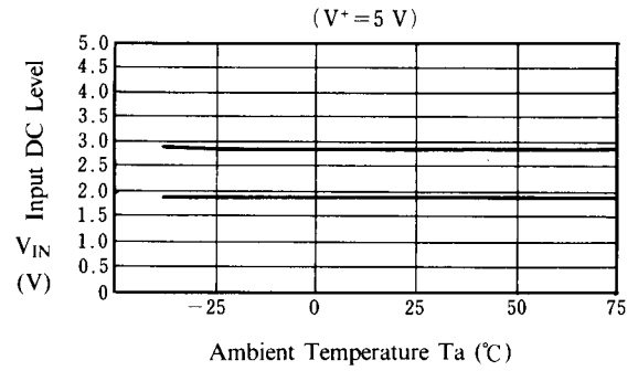
Input DC Level vs. Ta
