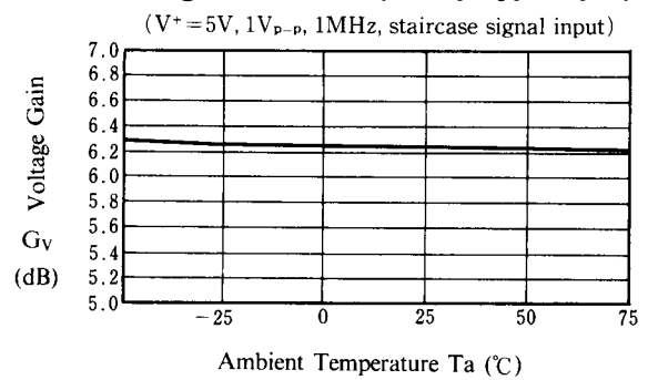
Voltage Gain vs. Ta (Clamp Type Input)
