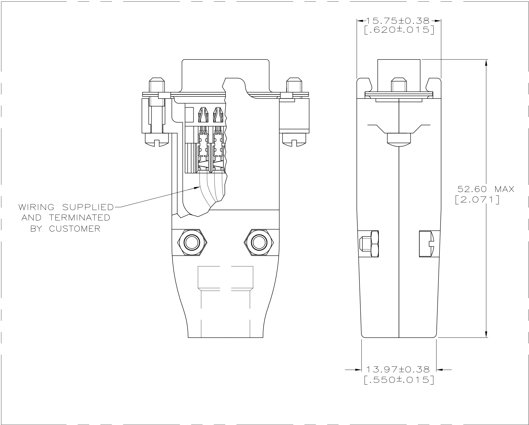
ASSEMBLED VIEW
