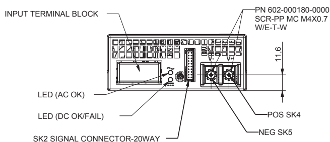
PSU Front View
