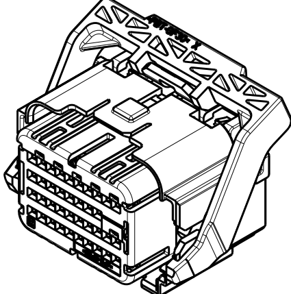
KEYING OPTION "G" SHOWN SEE SHEET 2 FOR BILL OF MATERIALS AND SHEET 3 FOR PIN-OUT CHARTS
