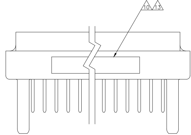
VIEW Z-Z
