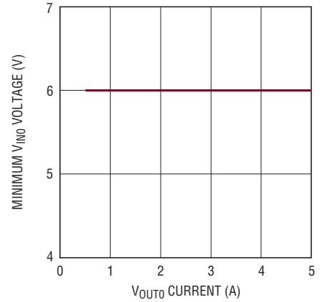
Minimum V_{\text{INO}} vs Output Current, V_{\text{OUTO}} = 3.3\text{V} and Below
