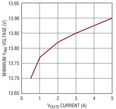
Minimum V_{\text{INO}} vs Output Current, V_{\text{OUTO}} = 12\text{V}
