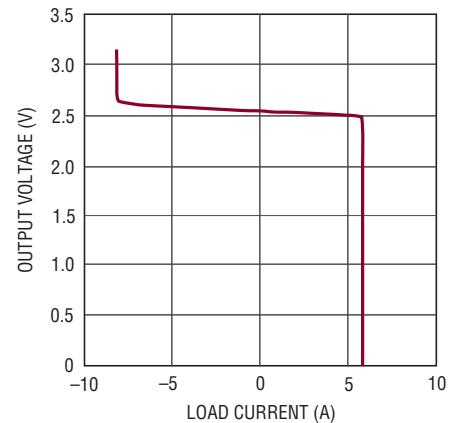
Output Voltage vs Output Current, V_{\text{OUTO}} = 2.5\text{V}
