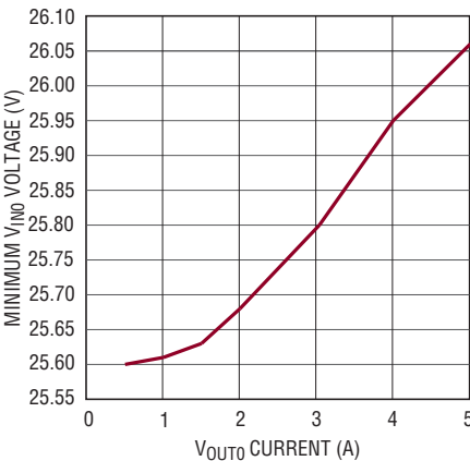
Minimum V_{\text{INO}} vs Output Current, V_{\text{OUTO}} = 24\text{V}
