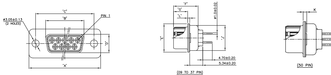
DIMENSION TABLE (RECEPTACLE CONNECTOR) :-
