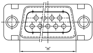
DIMENSION TABLE (PLUG CONNECTOR)
