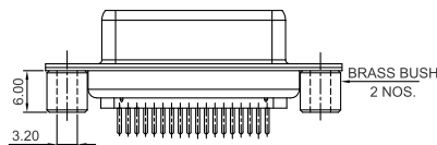
CONNECTOR WITH BRASS BUSH
