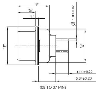
DIMENSION TABLE (PLUG CONNECTOR)
