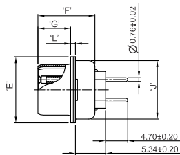
DIMENSION TABLE (RECEPTACLE CONNECTOR)
