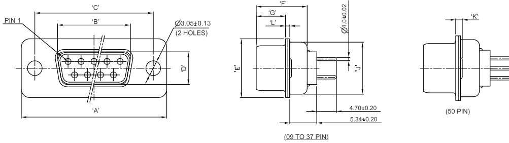
DIMENSION TABLE (PLUG CONNECTOR)
