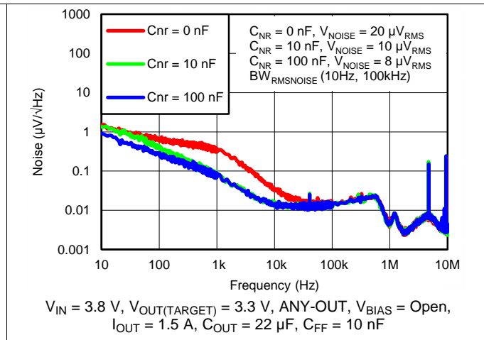
Figure 44. Spectral Noise Density vs C_{NR/SS}
