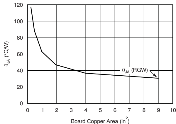
Figure 53. θ JA versus Board Size
