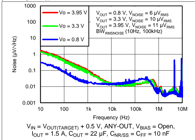
Figure 43. Spectral Noise Density vs Output Voltage
