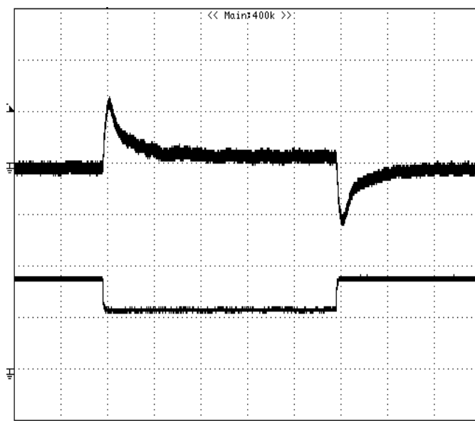
Figure 9: Output voltage response to step-change in load current (75%-50%-75% of I_o , max; di/dt = 2.5A/\mu s ). Load cap: 330\mu F , 35m\Omega ESR solid electrolytic capacitor and 1\mu F ceramic capacitor. Top Trace: V_{out} (100mV/div, 200us/div), Bottom Trace: I_{out} (5A/div). Scope measurement should be made using a BNC cable (length shorter than 20 inches). Position the load between 51 mm to 76 mm (2 inches to 3 inches) from the module
