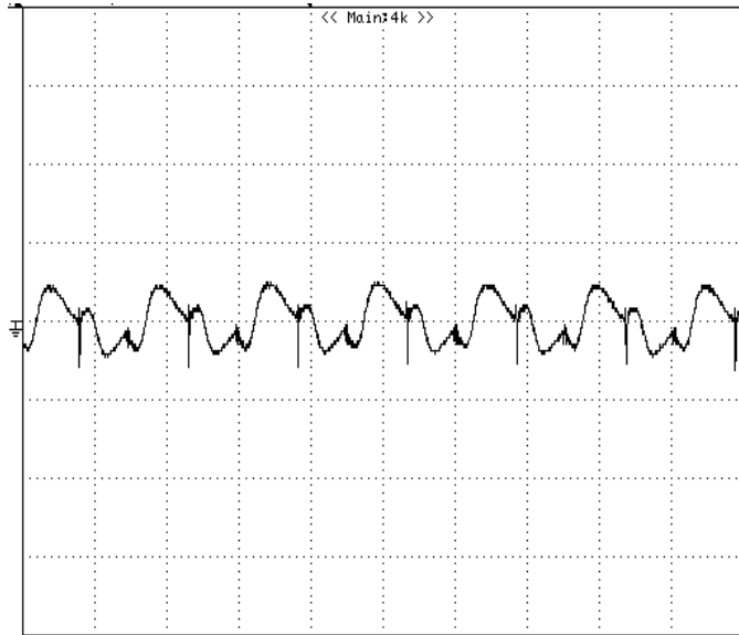
Figure 14: Output voltage ripple at nominal input voltage and rated load current ( I_o=12A ) (20 mV/div, 2 \mu s/div) Load capacitance: 1 \mu F ceramic capacitor and 10 \mu F tantalum capacitor. Bandwidth: 20 MHz. Scope measurements should be made using a BNC cable (length shorter than 20 inches). Position the load between 51 mm to 76 mm (2 inches to 3 inches) from the module
