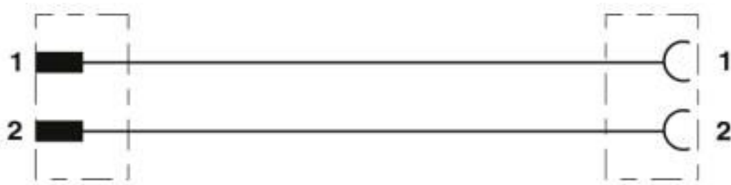
Contact assignment of the super seal plug to the super seal socket
