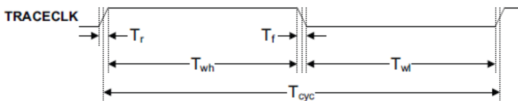
Figure 5. TRACE_CLKOUT specifications
