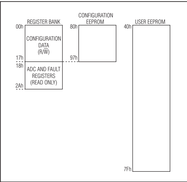
Figure 5. Memory Map
