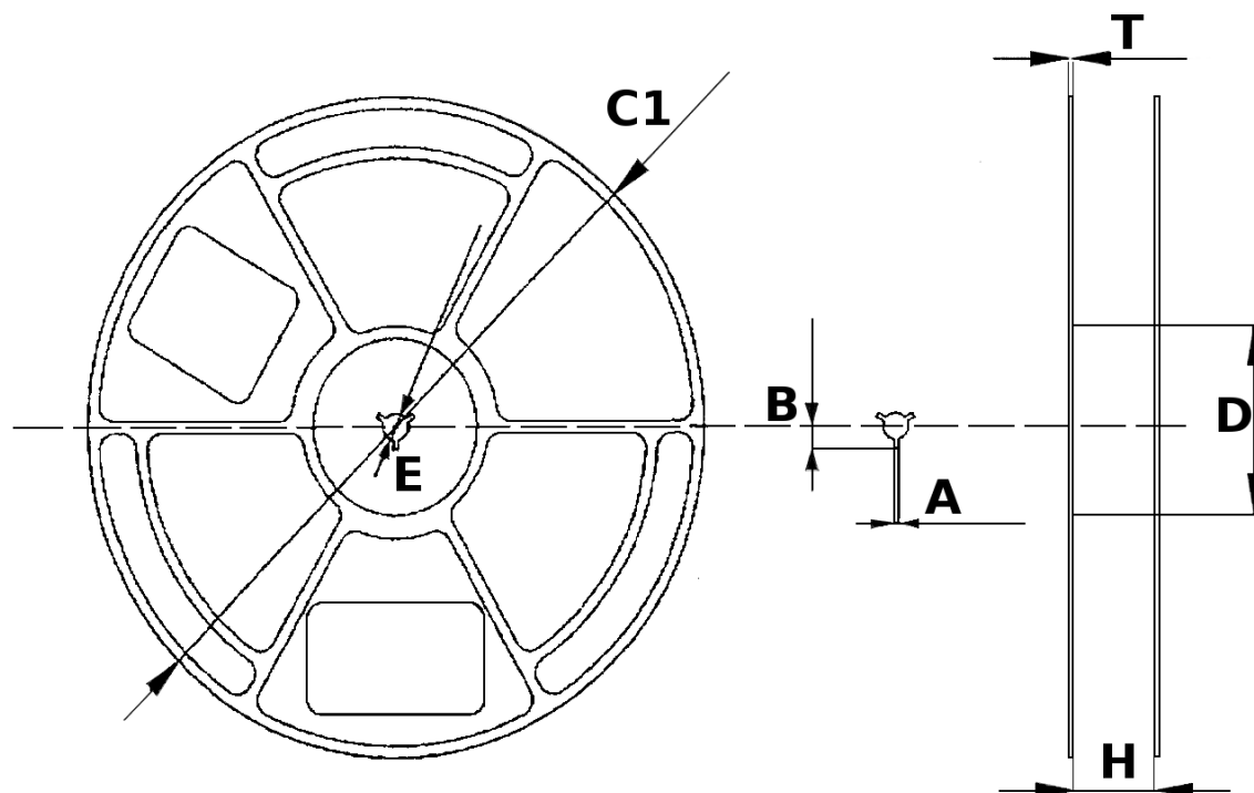
Figure 8 - Reel Specifications
