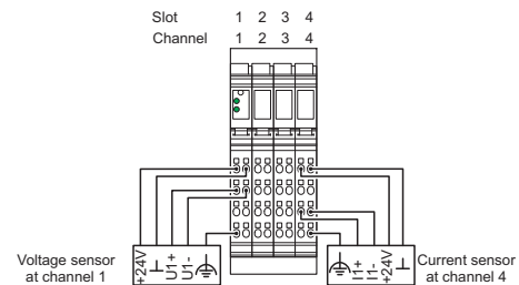
Connection diagram
