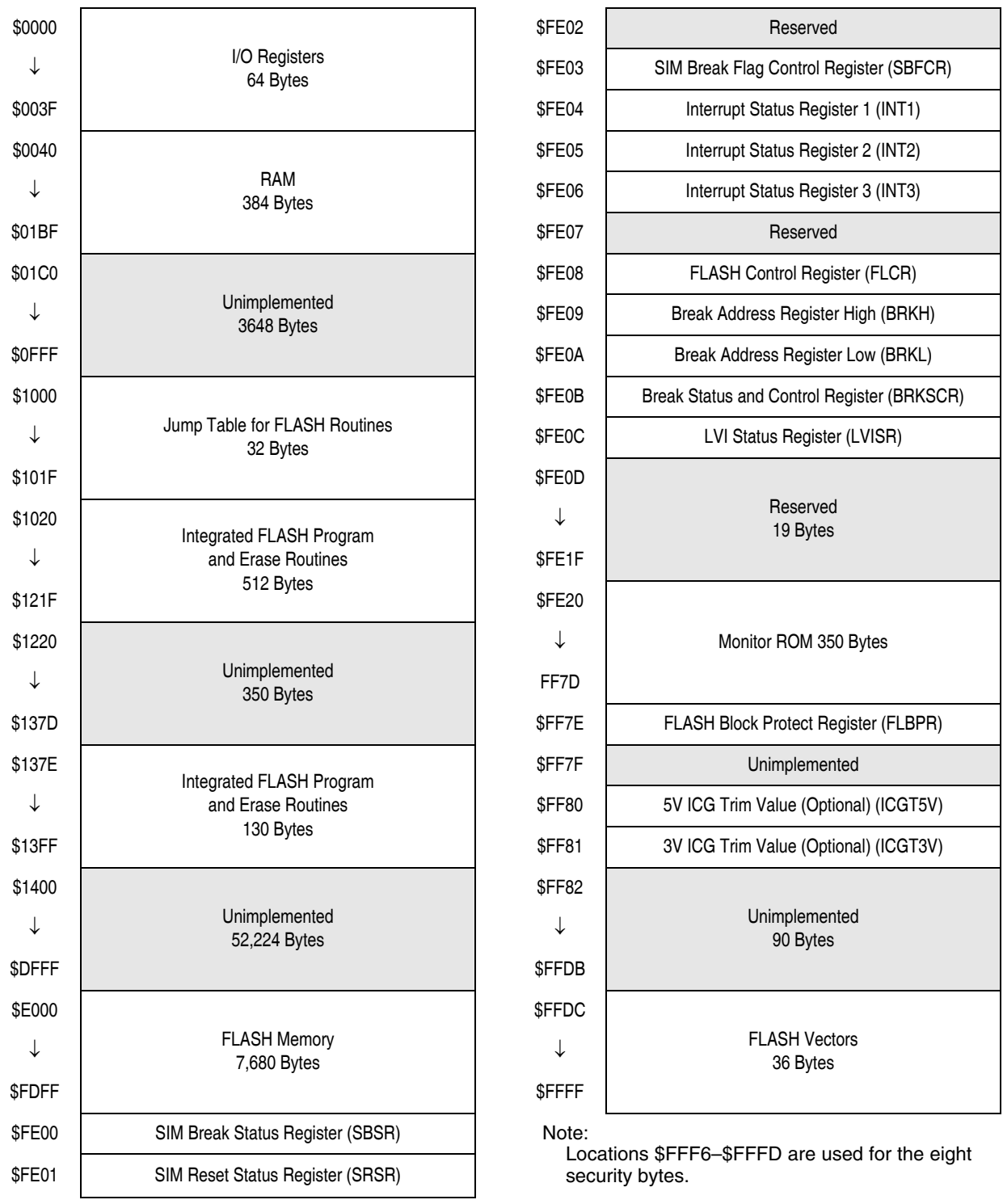
Figure A-2. MC68HC908EY8A Memory Map
