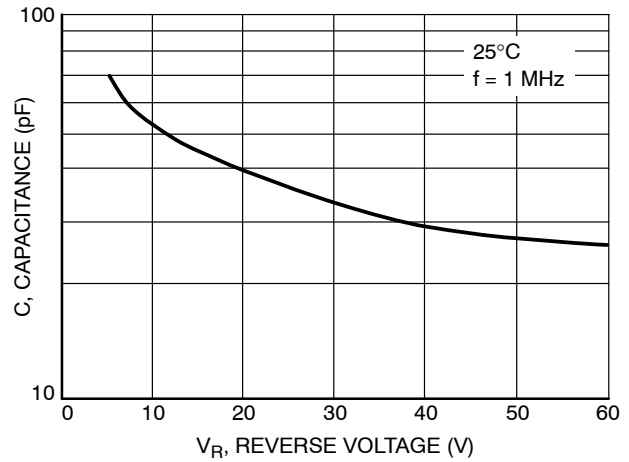
Figure 4. Typical Capacitance
