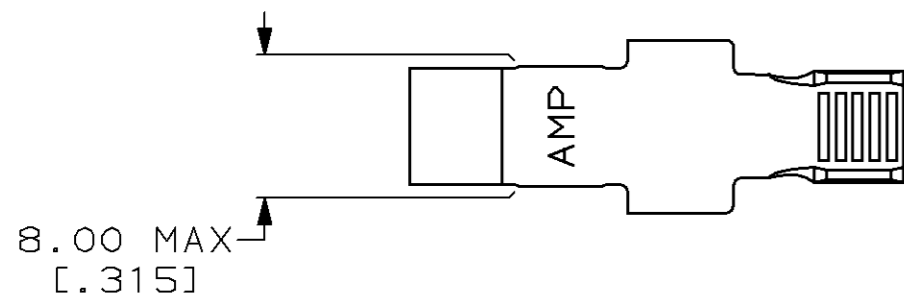
DETAIL C
