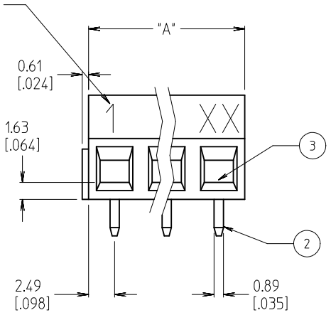
3 CIRCUIT SHOWN
