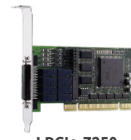
LPCle-7250
