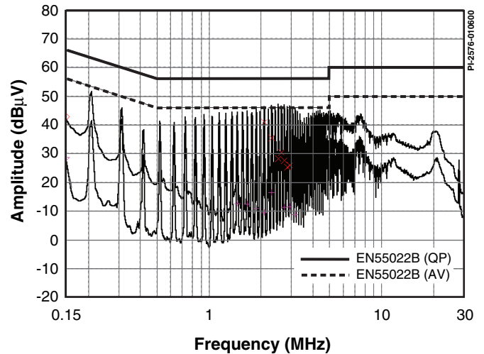
Figure 13. Fixed Frequency Operation Without Jitter.
