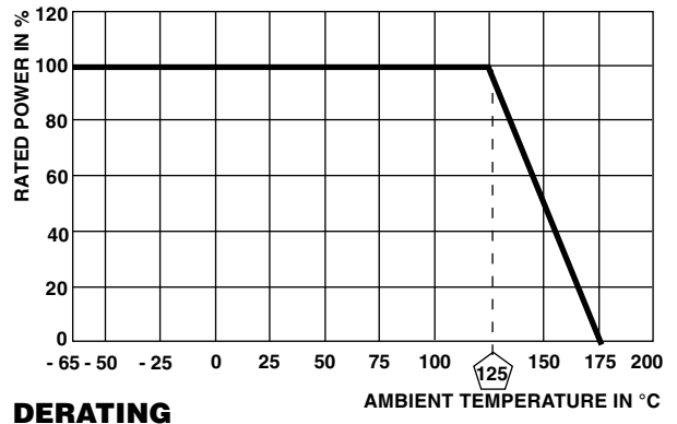
DERATING
