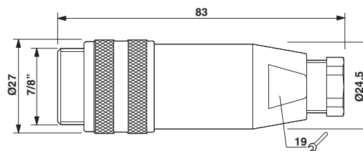
Dimensional drawing
