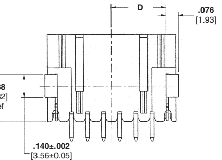
Section K-K
