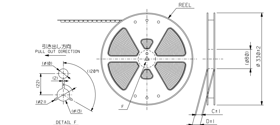
DETAIL F
