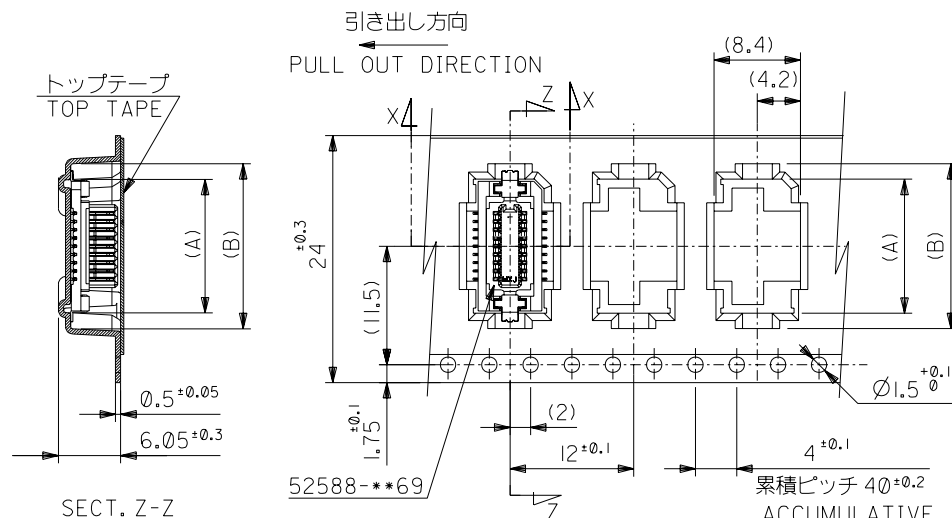
SECT. Z-Z
