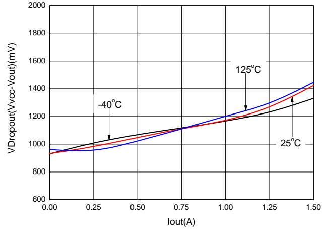
Figure 10 V_{CC} Dropout Voltage vs. I_{OUT} and Temperature ( T_A )
