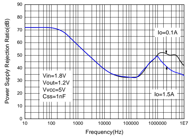
Figure 12 V_{CC} PSRR vs. Frequency
