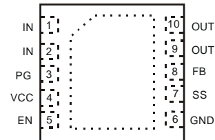
DFN3030-10
