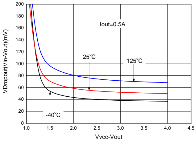
Figure 9 V_{IN} Dropout Voltage vs. (V_{CC}-V_{OUT}) and Temperature ( T_A )
