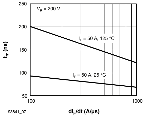
93641_07 di_F/dt (A/μs) Fig. 7 - Typical Reverse/dt Recovery Time vs. di_F/dt
