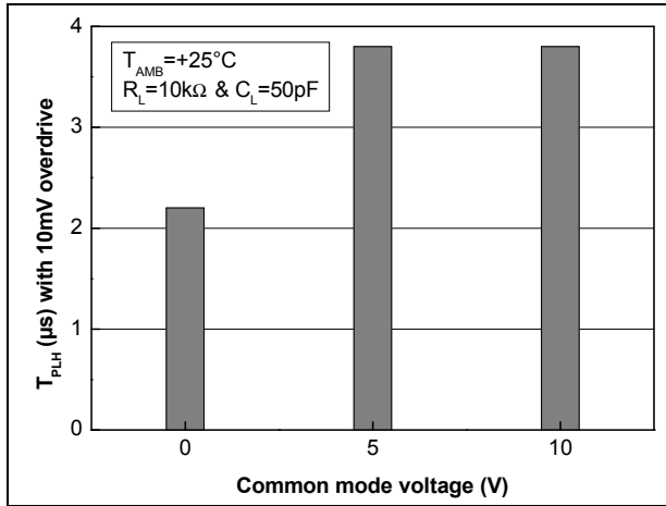
Figure 7. T_{PLH} vs V_{icm} at V_{CC} = 10\text{ V} and 10 mV overdrive
