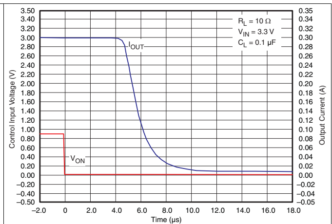
Figure 23. t_{OFF} Response
