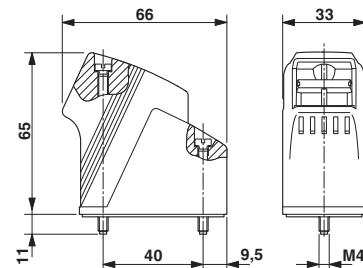
Dimensional drawing
